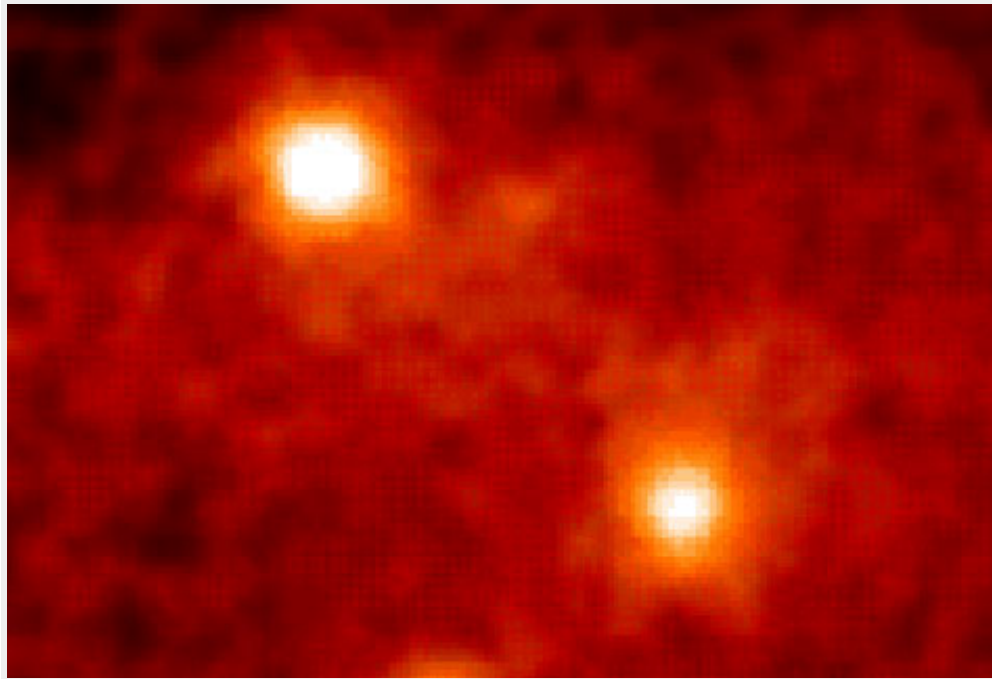
Image of the Crab Nebula and nearby region as seen in gamma ray wavelengths.
