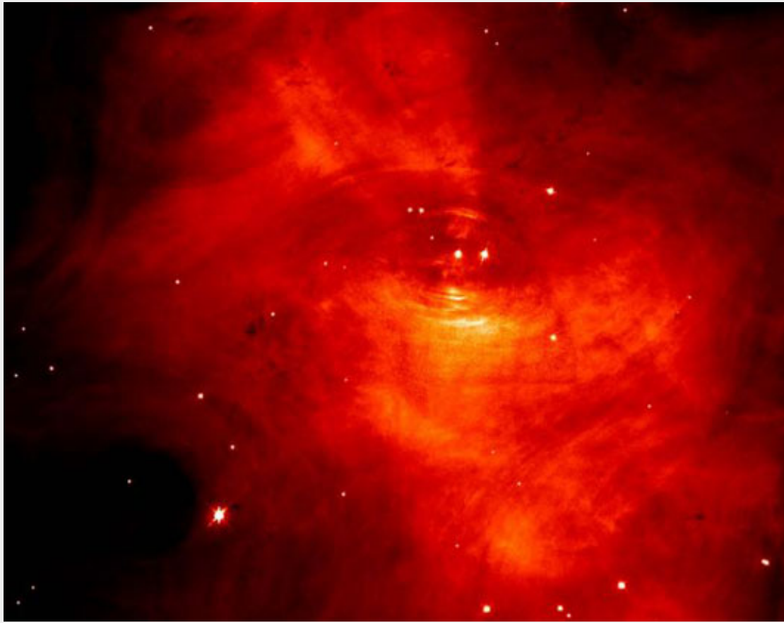
Image of the Crab Nebula taken in visible light with the Hubble Telescope
