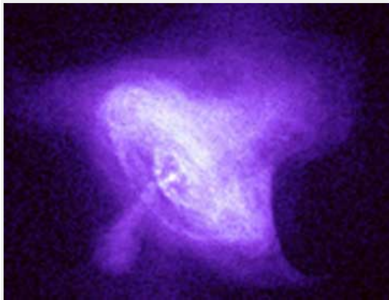
Crab Nebula images in x-rays by NASA's Chandra Observatory.
